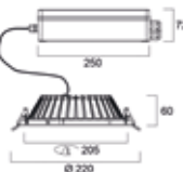
Insaver Slim 205 IP65
